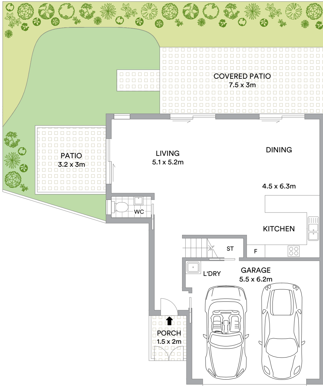
GROUND FLOOR
