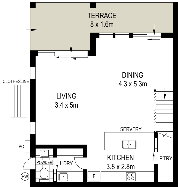
GROUND FLOOR (TYPE A)
