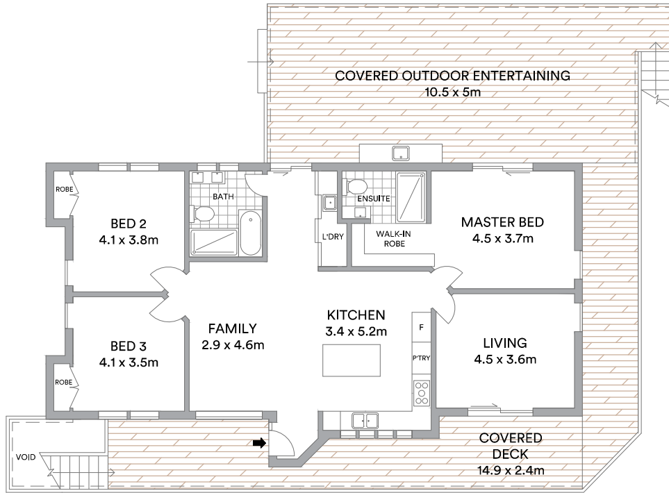
UPPER FLOOR
