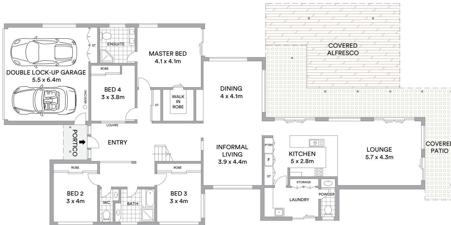
GROUND FLOOR
