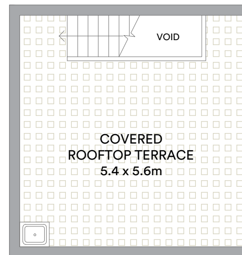
LEVEL SEVEN
