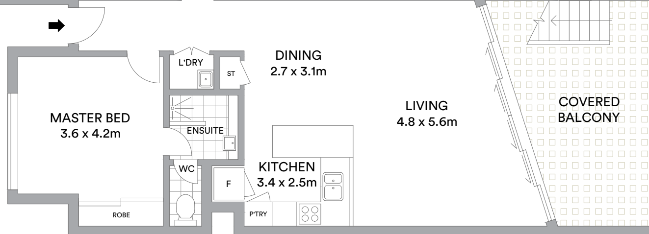
LEVEL SIX
