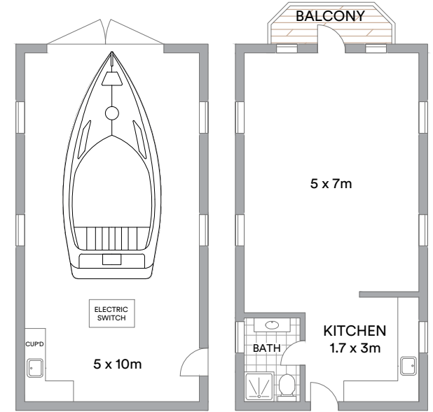
GROUND LEVEL (BOAT HOUSE)
