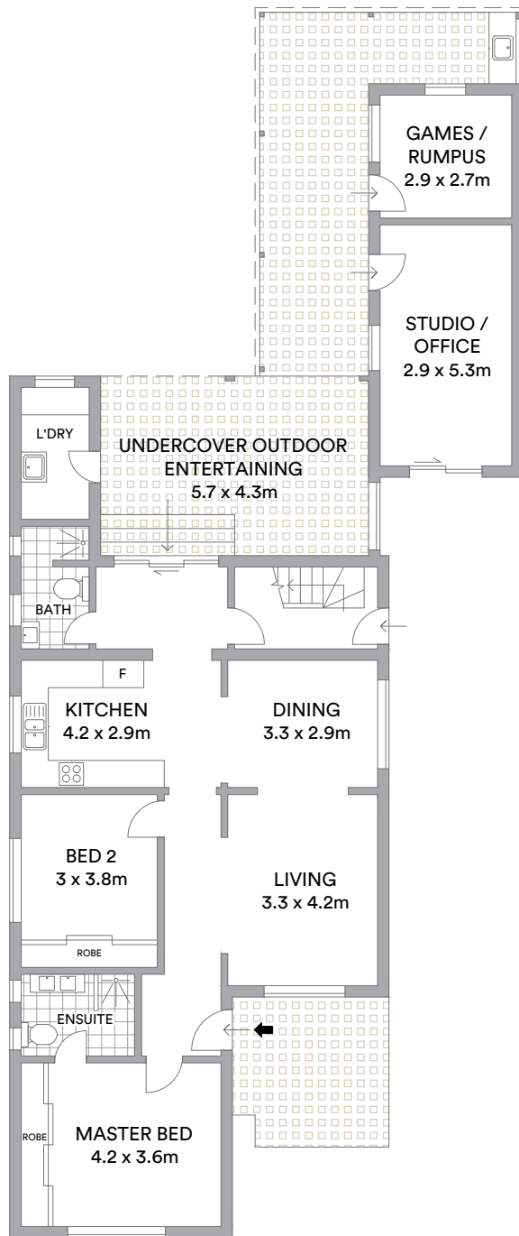
GROUND FLOOR
