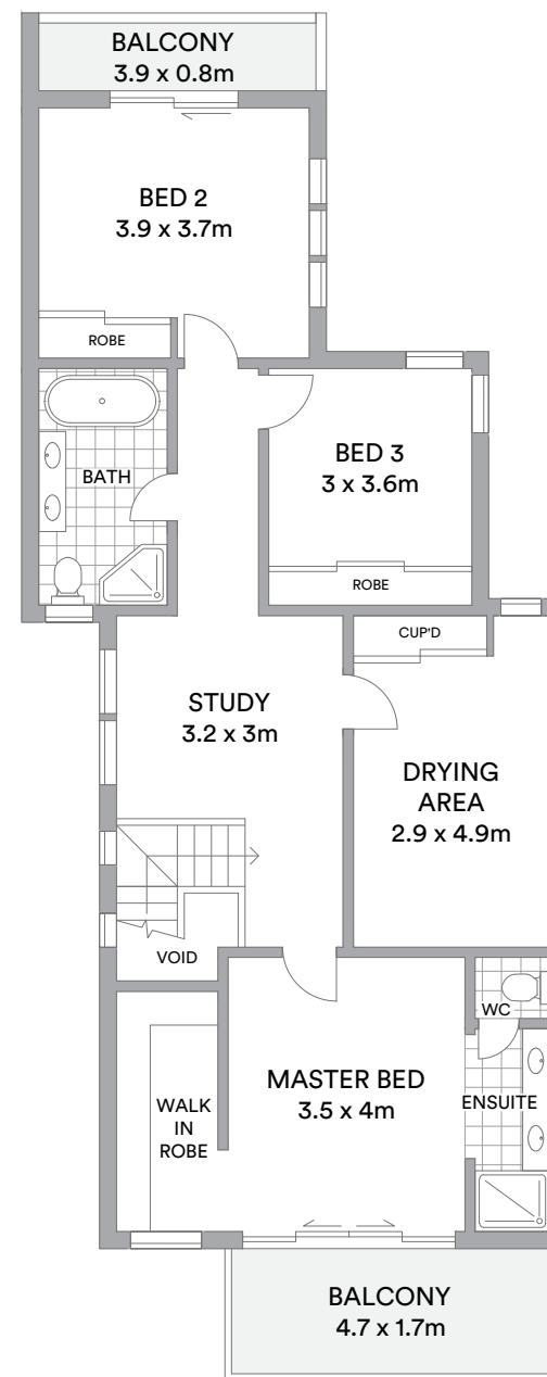
FIRST FLOOR
