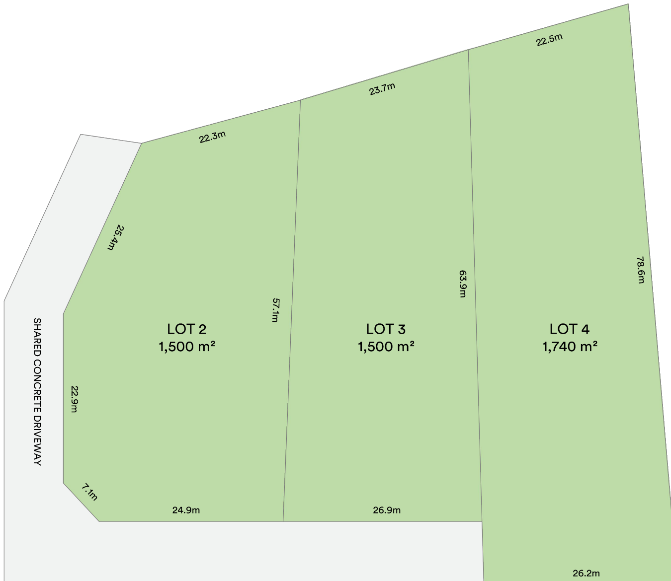
SITE PLAN
