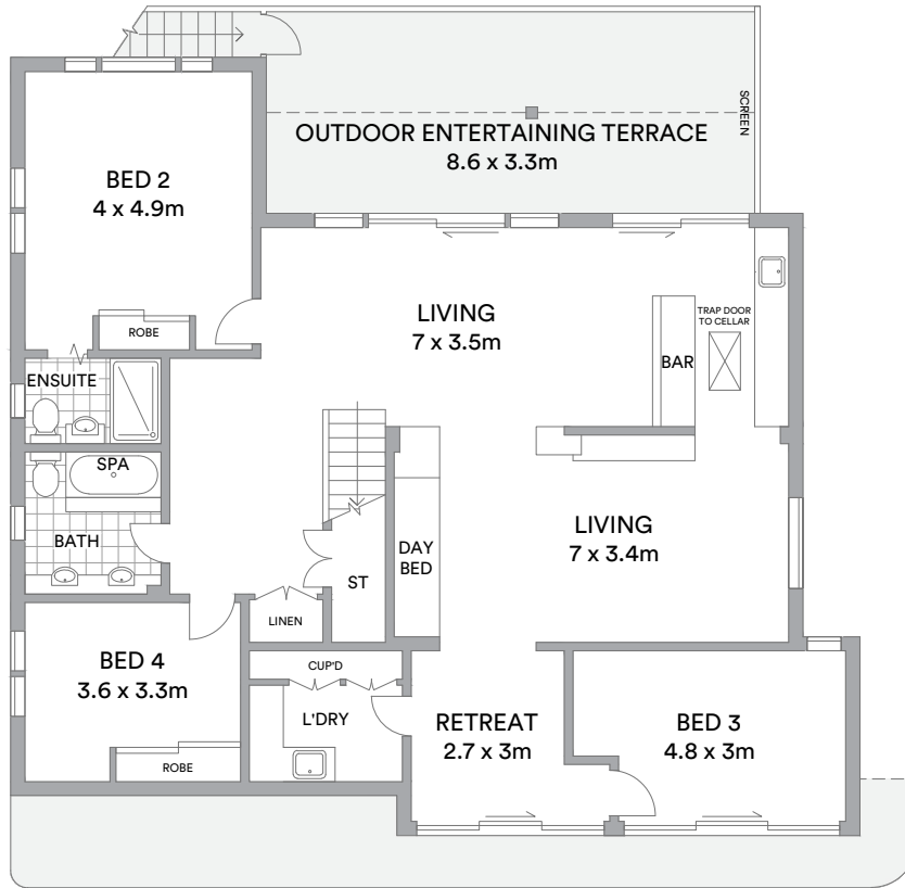
LOWER LEVEL
