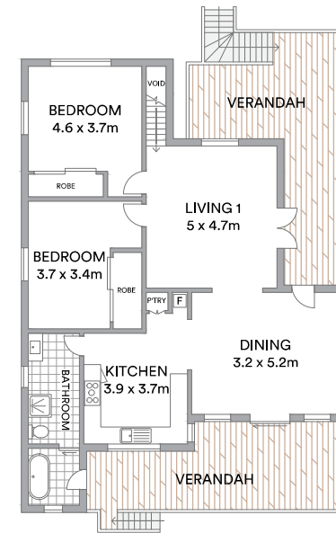
UPPER FLOOR
