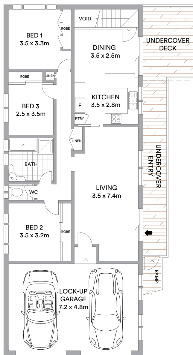
ENTRY LEVEL
