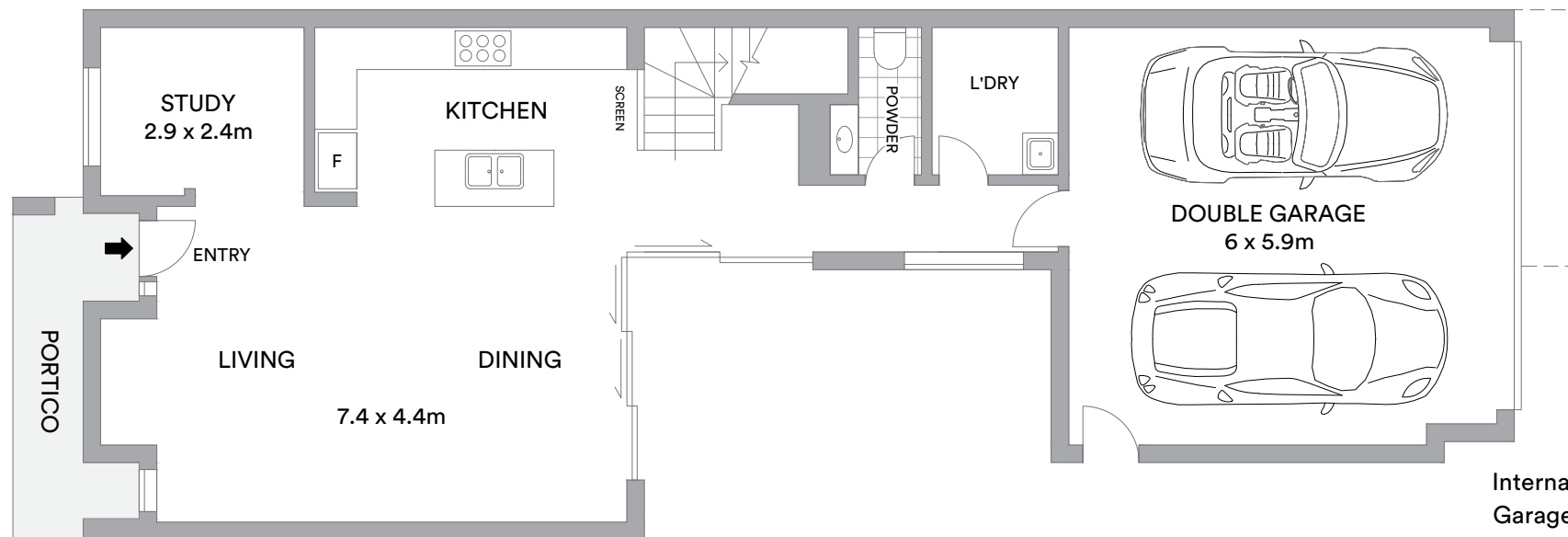
GROUND FLOOR
