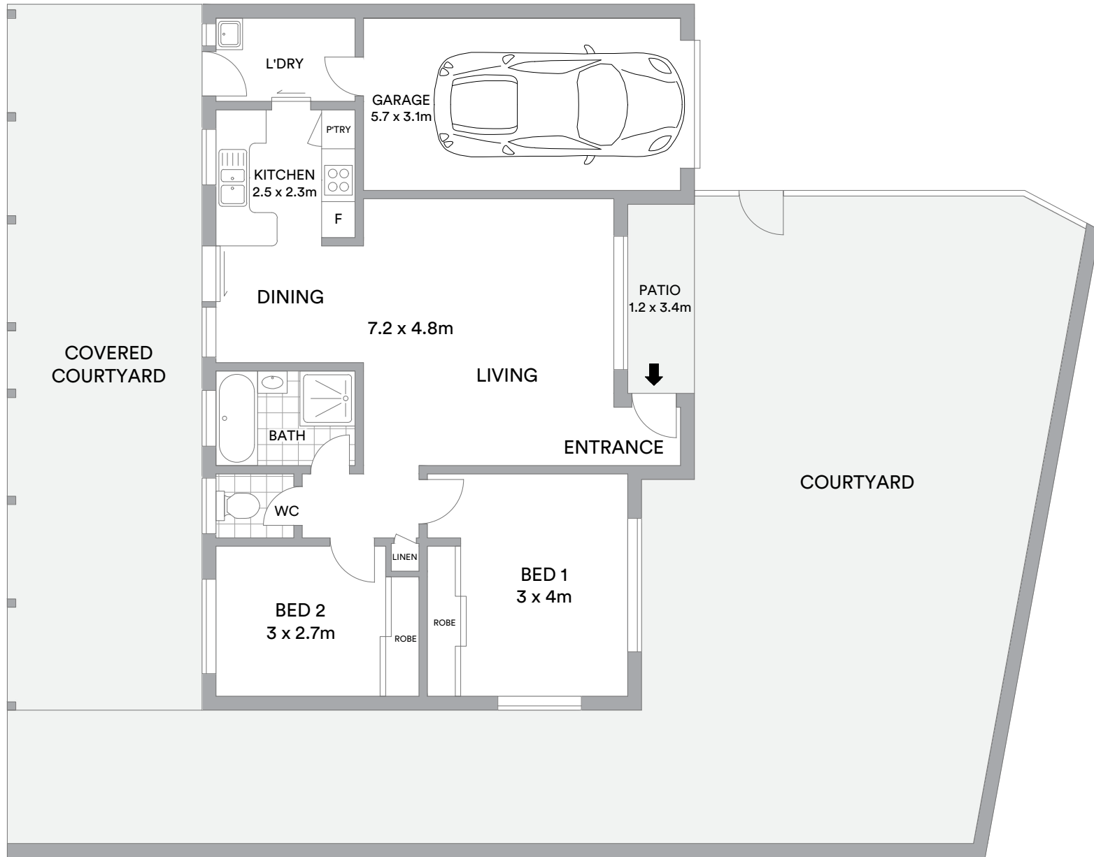
GROUND FLOOR
