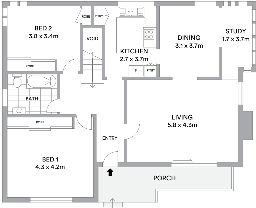
ENTRY LEVEL
